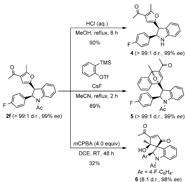
Scheme 3. Further transformation of 2f . m CPBA = m -chloroperbenzoic acid, Tf = trifluoromethanesulfonyl, TMS = trimethylsilyl.
