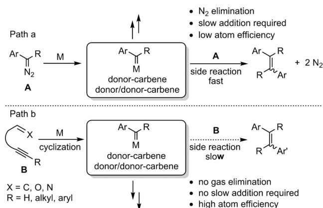
Scheme 2. Carbene chemistry based on different approaches.
