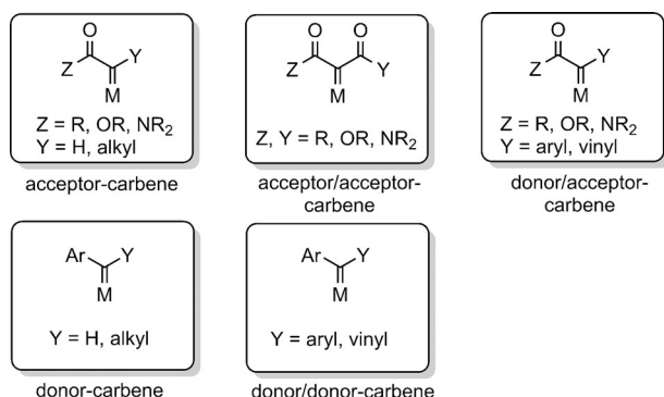
Scheme 1. Different types of metal carbenoids.
